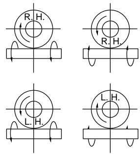
ROTATION FACING COVER AND END OF SHAFT
